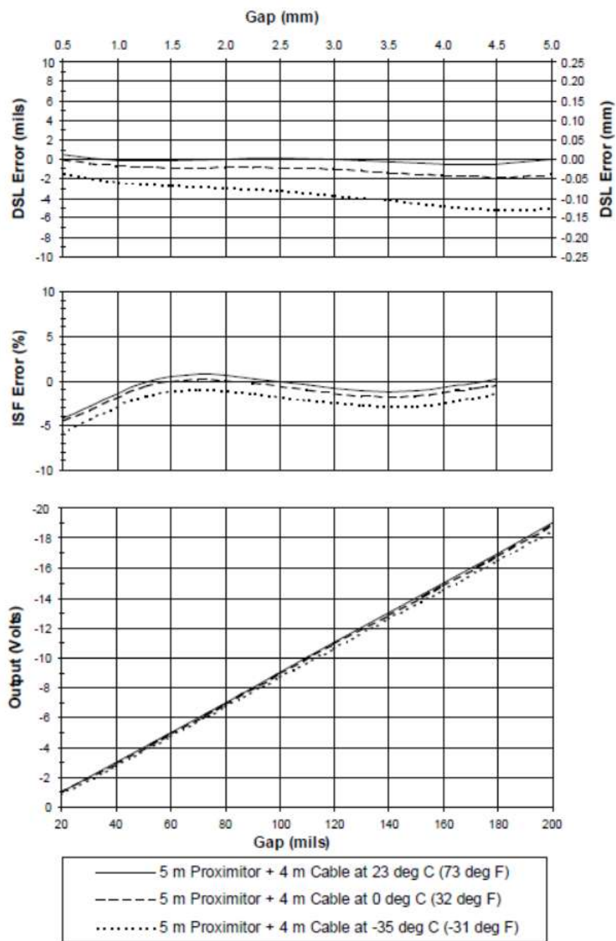
Figure 5: Typical 3300 XL 11 mm 5 m Proximitor Sensor with 4 m of Extension Cable @ Cold Temperature
