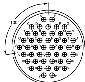
100° Rotation of 36-10
