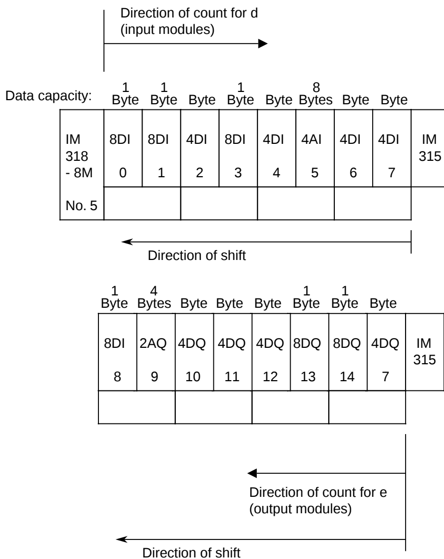
Figure 4-7 ET 100U Configuration for Calculating the Transmission Time
