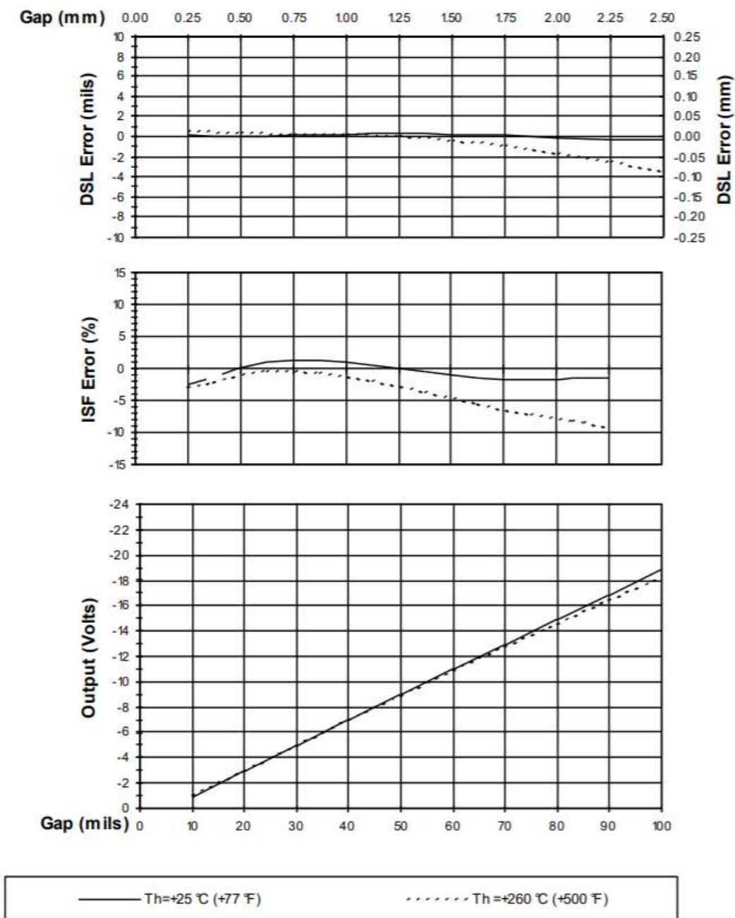
Figure 8: Typical 3300 XL Extended Temperature Range Probe and 4 m Extended Temperature Range Extension Cable at T_h (Proximitors Sensor and Probe Tip with 1-foot Cable are at +25°C)
