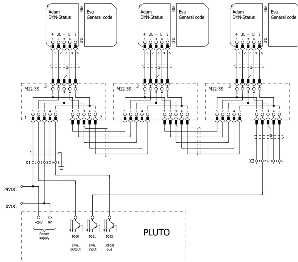
A) Three Adam DYN-Status connected to a Pluto Safety PLC via M12-3S to use StatusBus.
